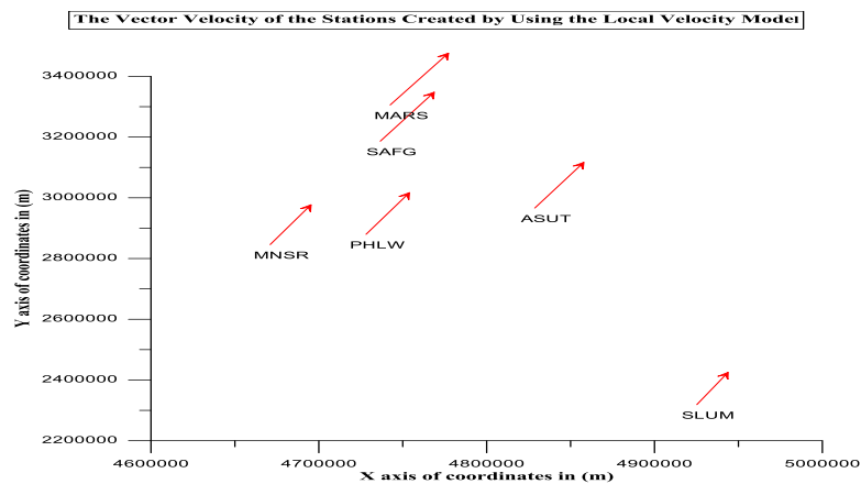
Figure (8): The Velocities Vector Length of the Stations Computed by Using the Mean Local Velocity Model.
