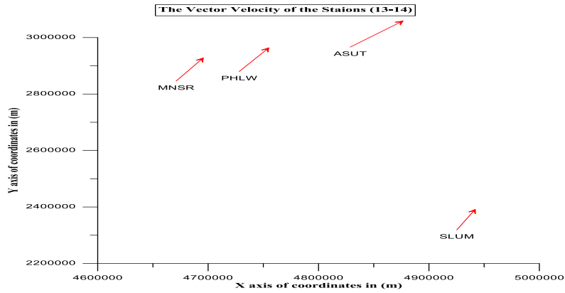
Figure (7): The Velocities Vector Length of the Stations Computed by Using the GPS Observations at (2013 and 2014).
